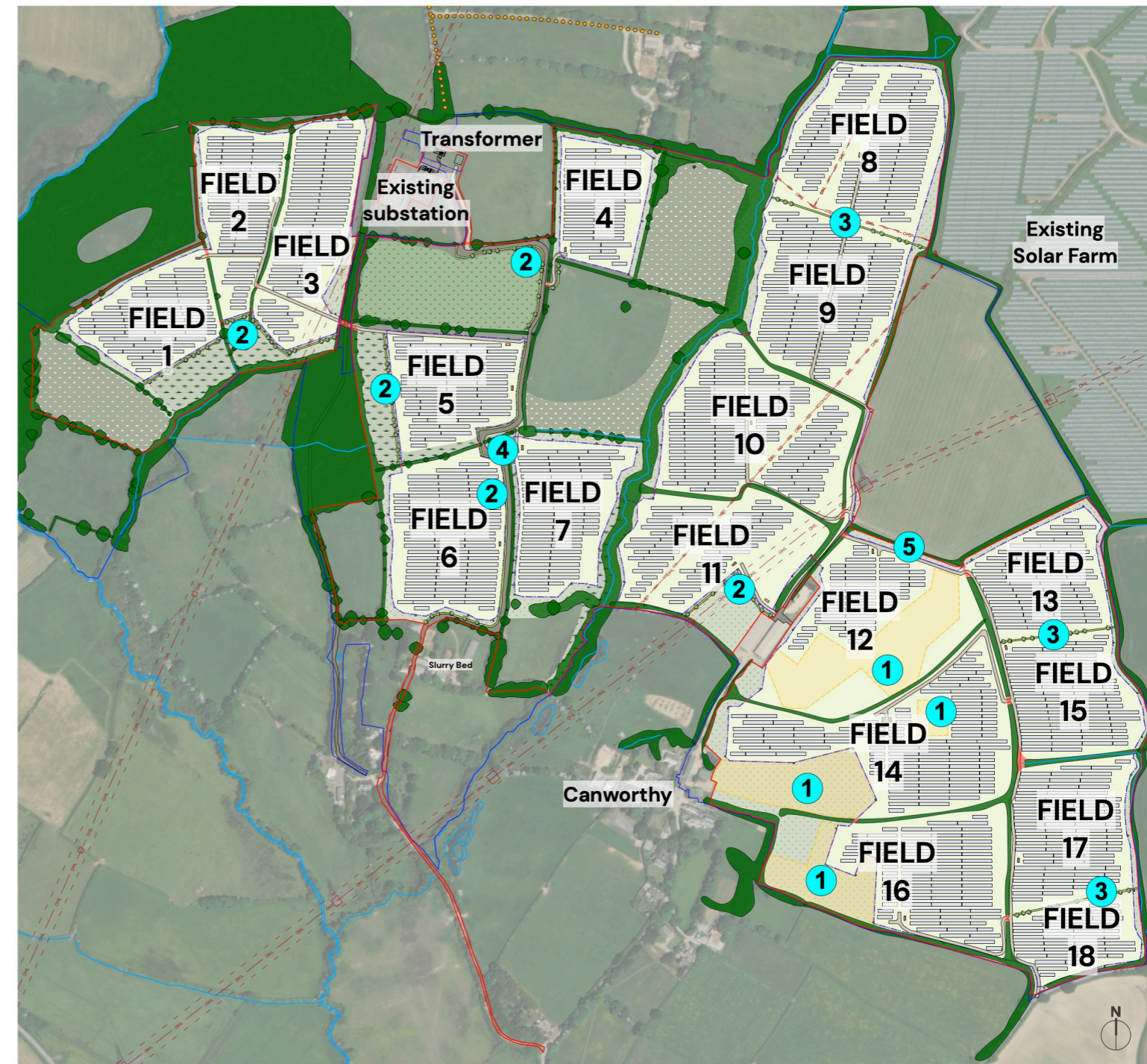
P24-2210_EN_20 - AMENDED SCHEME LANDSCAPE & ECOLOGICAL MASTERPLAN (not to scale)
